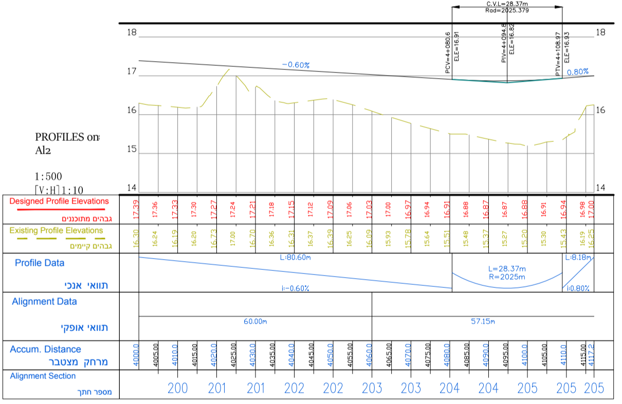
Road [AI2] Scale 1:50\500
