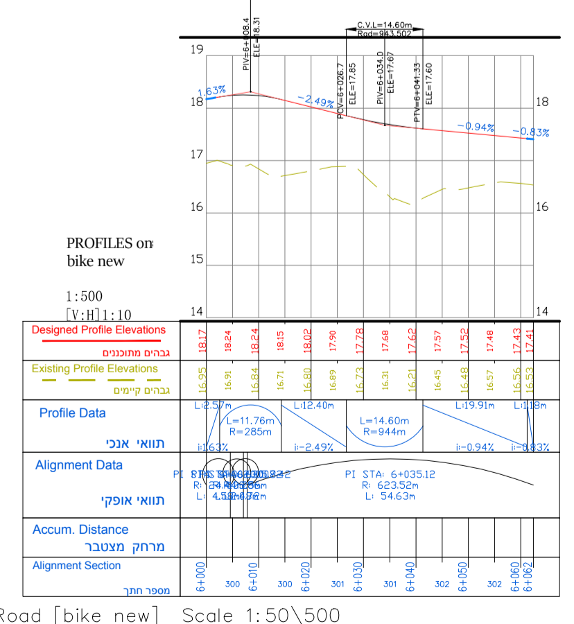
Road [bike new] Scale 1:50\500
