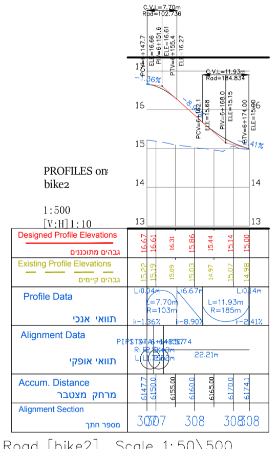
Road [bike2] Scale 1:50\500
