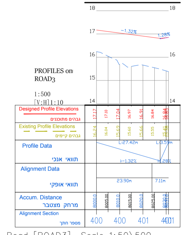
Road [ROAD3] Scale 1:50\500
